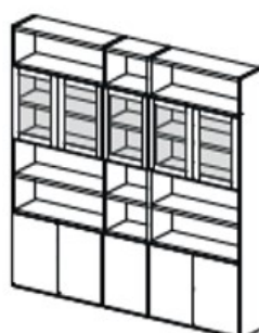
CM13 2280x330x2272H
