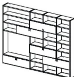
CM42 3030x330x2272H
