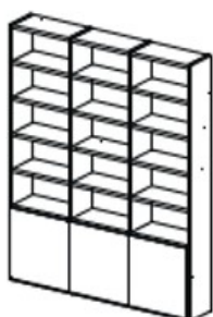
CM11 1830x330x2272H
